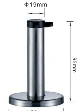
DH032 Stainless steel SIZE: \phi 50 \times 95 mm
