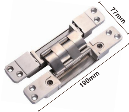
AG02 Three dimensional adjustable concealed hinge SIZE:29×190mm
