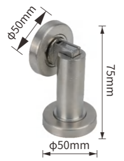
DH045 Stainless steel investment casting SIZE: \phi 50 \times 75mm
