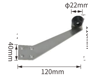
DH028 Stainless steel Right coat hook SIZE: 120 \times 110 mm
