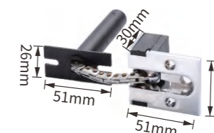
FM13 Zinc alloy SIZE:51×43×30mm
