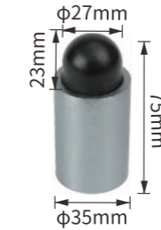
DH067 Aluminium alloy SIZE: \phi 35 \times 75mm
