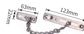
FM09 Stainless steel SIZE:123×63×22mm
