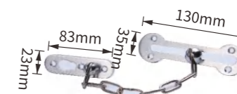
FM07 Zinc alloy SIZE:130×35mm 83×23mm
