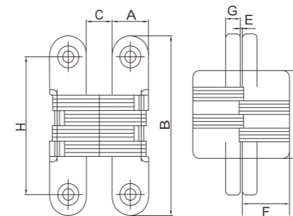
Outline dimensions of dark hinge
