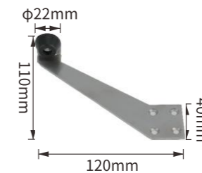
DH027 Stainless steel Left coat hook SIZE: 120 \times 110 mm
