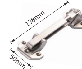
FM04 Zinc alloy SIZE:138×50mm
