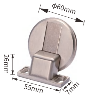
DH050 Stainless steel investment casting SIZE: \phi 60 \times 55 \times 7mm
