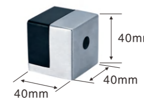
DH078 Stainless steel investment casting SIZE: 40 \times 40 \times 40mm
